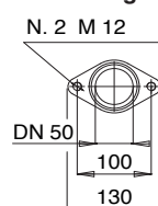
Oval Flanges
